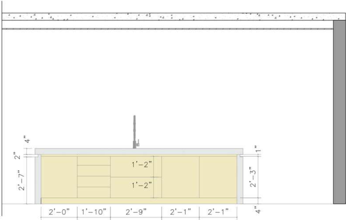
KITCHEN - ELEVATION 3 1:25
