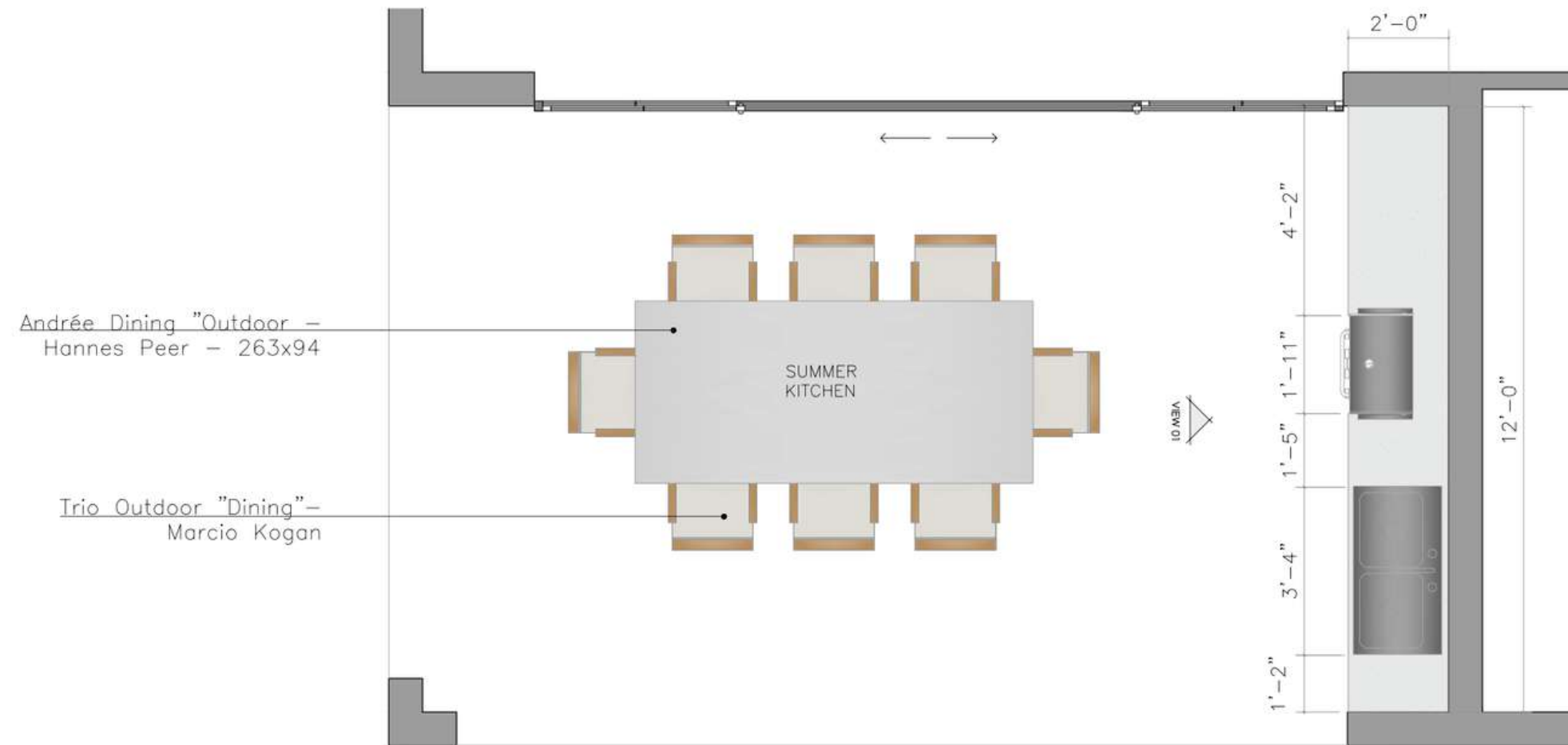
SUMMER KITCHEN - FLOOR PLAN 1:25
