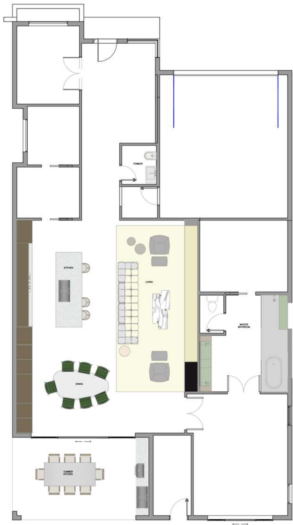
FLOOR PLAN 1:75
