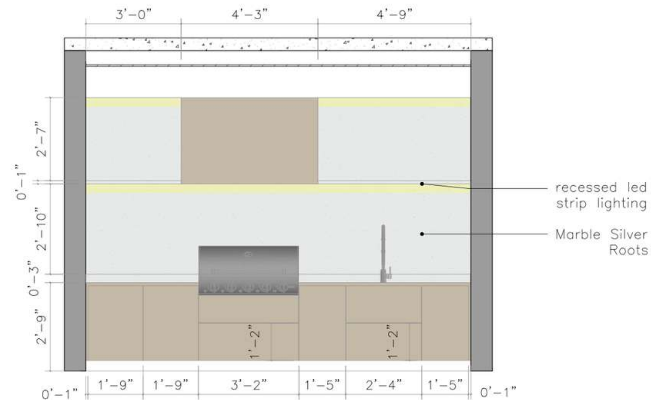
SUMMER KITCHEN - ELEVATION 1 1:25
