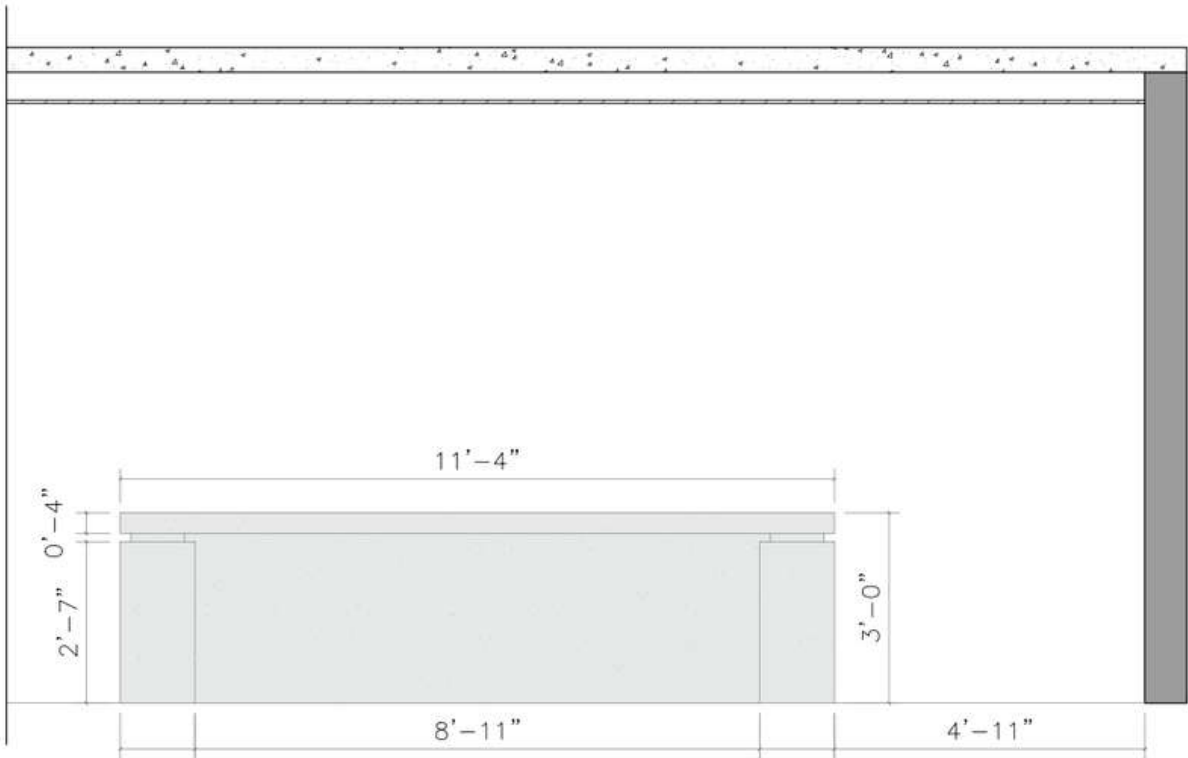
KITCHEN - ELEVATION 4 1:25
